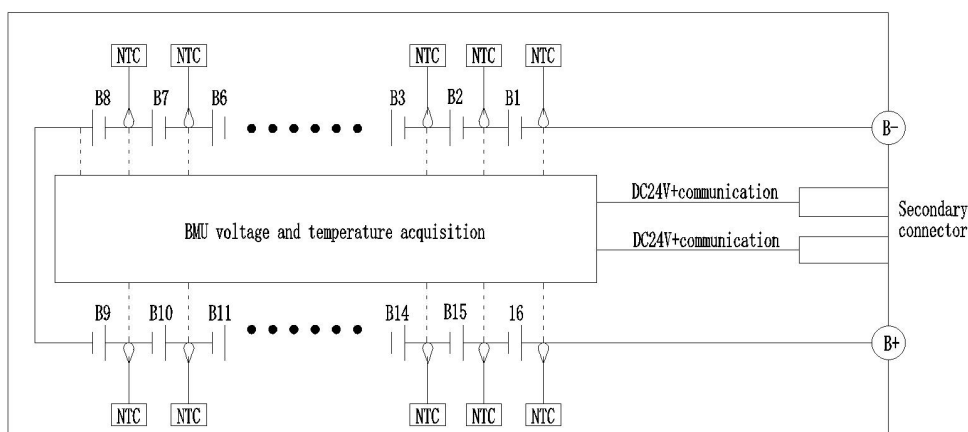
Electrical schematic diagram of battery module
