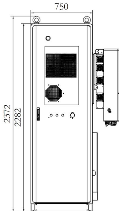
Front View
