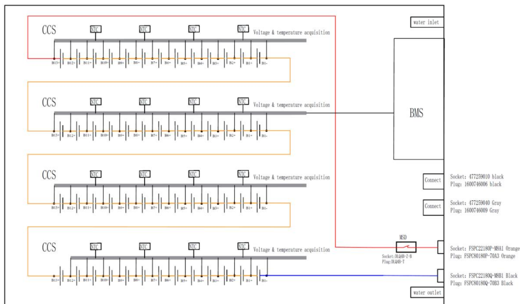
Liquid cooled battery module 1P52S 166.4V280AH
